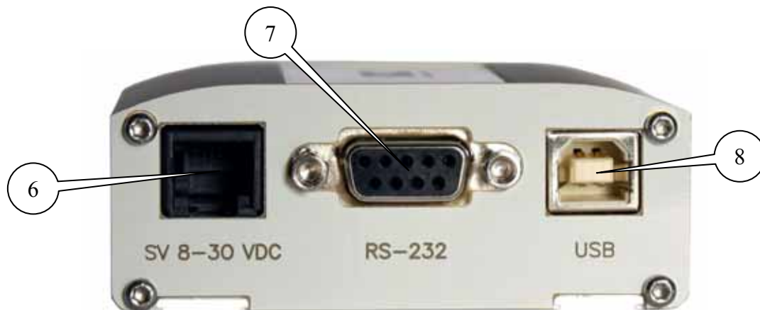
Fig.1.4.1 Front view
