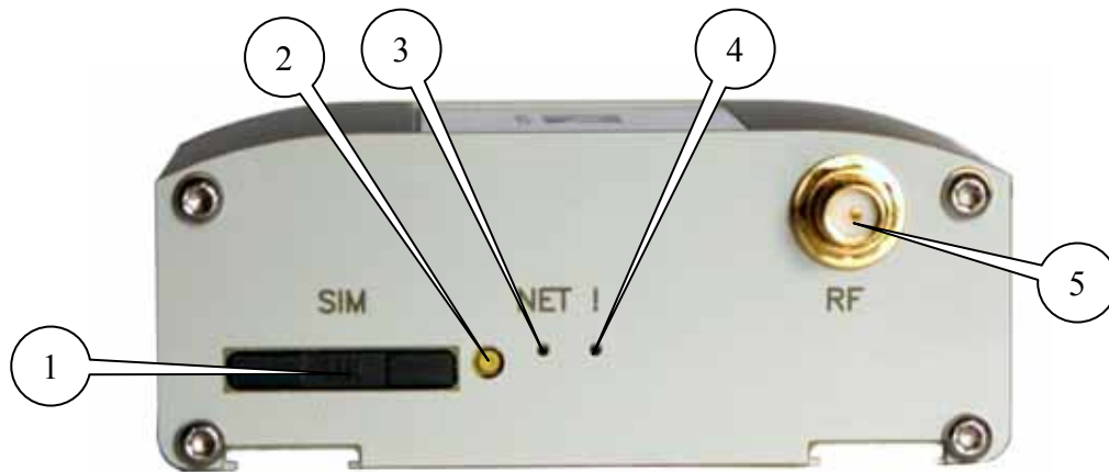
Fig.1.4.1 Front view
